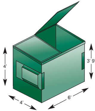
3-Yard Bin
